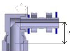
Pag. 10/11 - "O" ring female swivel, 90° blocktype
